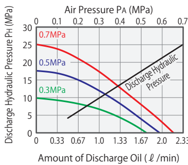
AB6000 Calculation Formula P_H = 38(P_A - 0.04)
