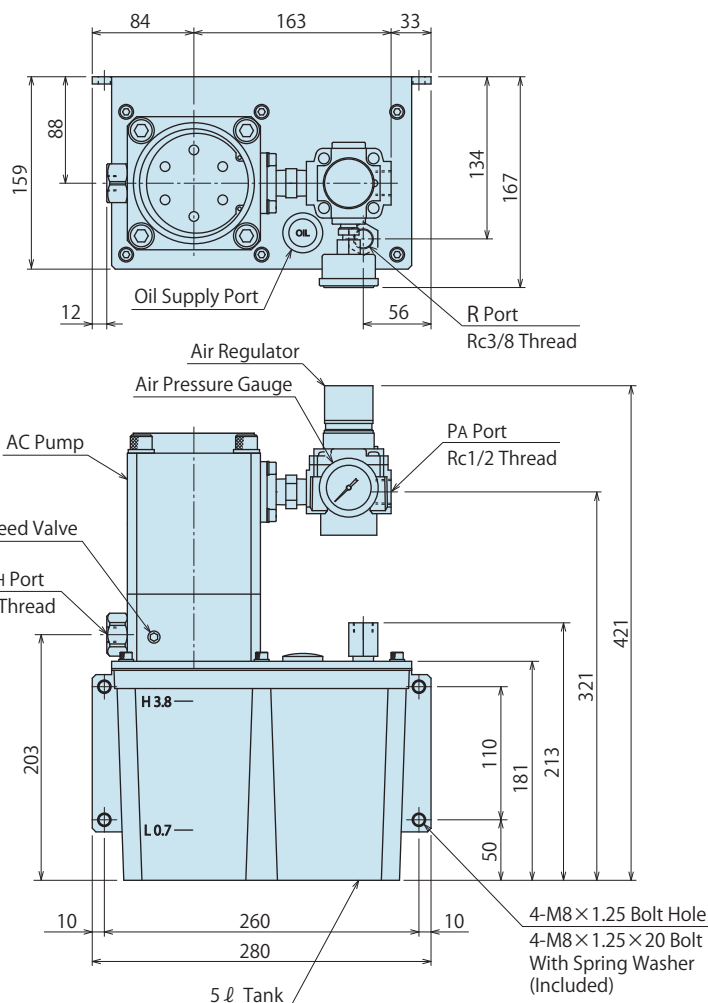
BH Non-Leak Valve Unit
