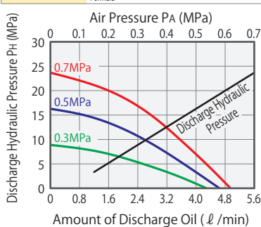
AC9001 Calculation Formula P_H = 147(P_A - 0.06)
