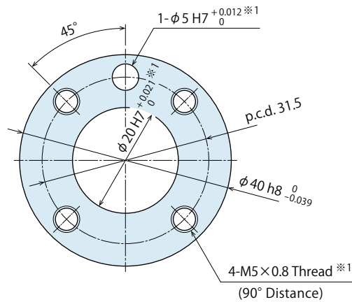
Mounting Pattern Number : 2
