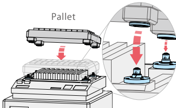
Pneumatic Location Clamp model SWQ/SWT
