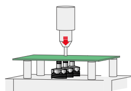
High-Power Pneumatic Work Support model WNC
