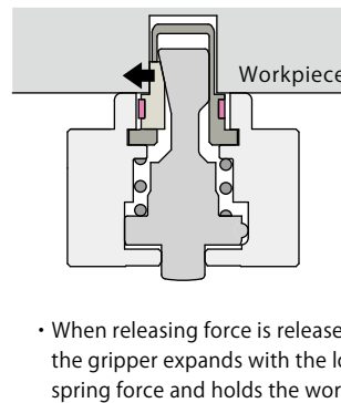
Holding a Workpiece (Lock)
