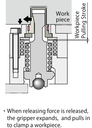
Clamping a Workpiece (Lock)
