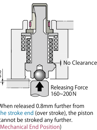
(Mechanical End Position)
