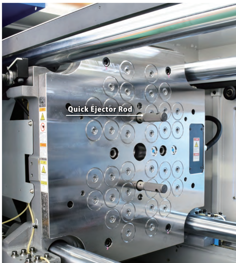
Machine Capacity : 100-ton class, Magnetic Plate : MAG010□ (Plate Thickness 35mm, The Number of Discharges : 1, Applicable Temperature 120°C, Detection System : MIMS&DMS) Level Unit : Maximum Mold Loading Weight 0.7-ton model
