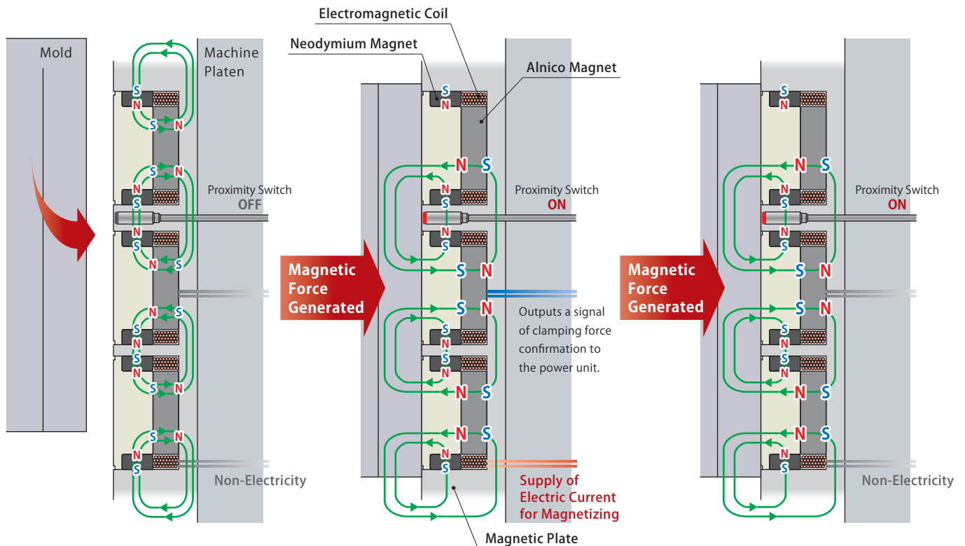
De-Magnetized
