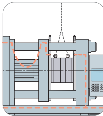
During Magnetization
